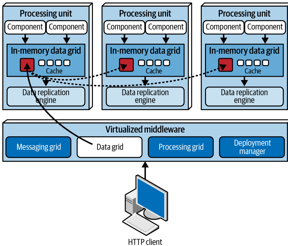
Figure 16-5. The data grid synchronizes the in-memory caches
