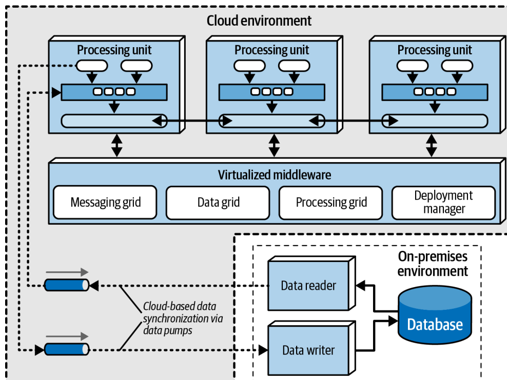
Figure 16-14. Hybrid cloud-based and on-prem topology
